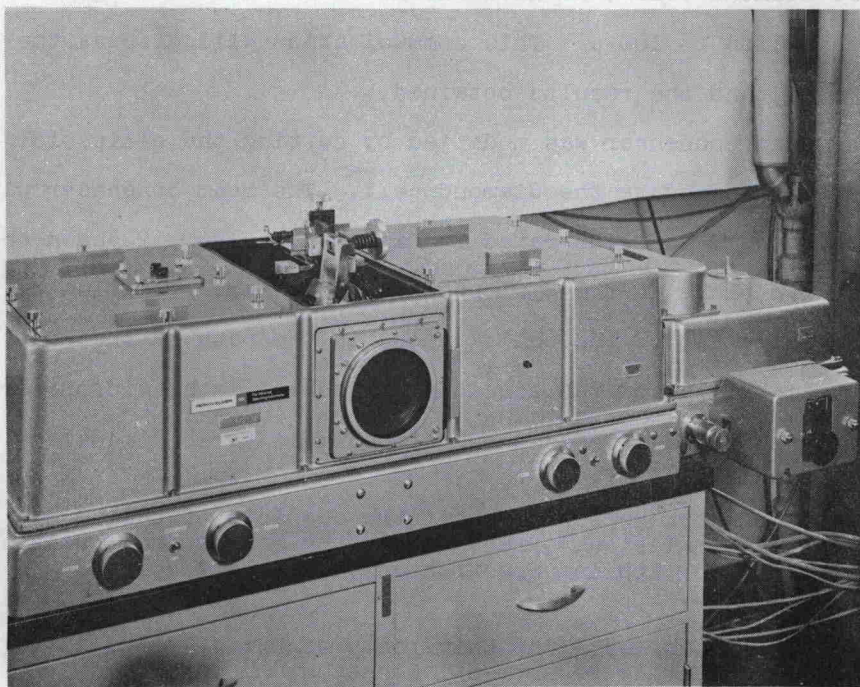
Fig. 2 - High pressure cell in the Perkin-Elmer #301 far infrared spectrophotometer.
